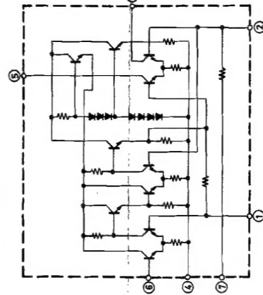
IC102 (TA7061AP)
